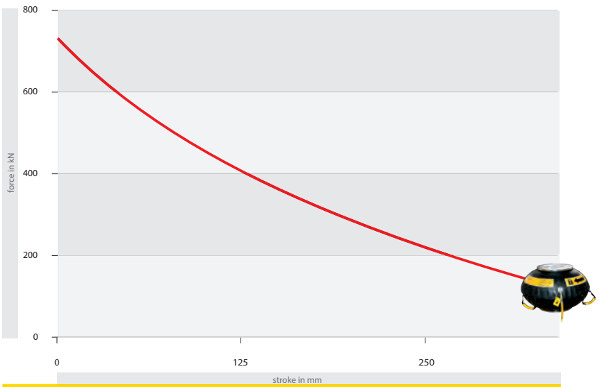
Load path diagram VCB 75
